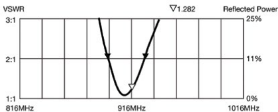
The Linx ANT-916-CW-HWR-RPS antenna is used for 908...917, 919...921 MHz (ZMEURAZBERRY7_ANT)
