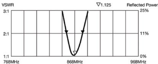
The Linx ANT-868-CW-HWR-RPS antenna is used for 865...869 MHz (ZMEERAZBERRY7_ANT)
